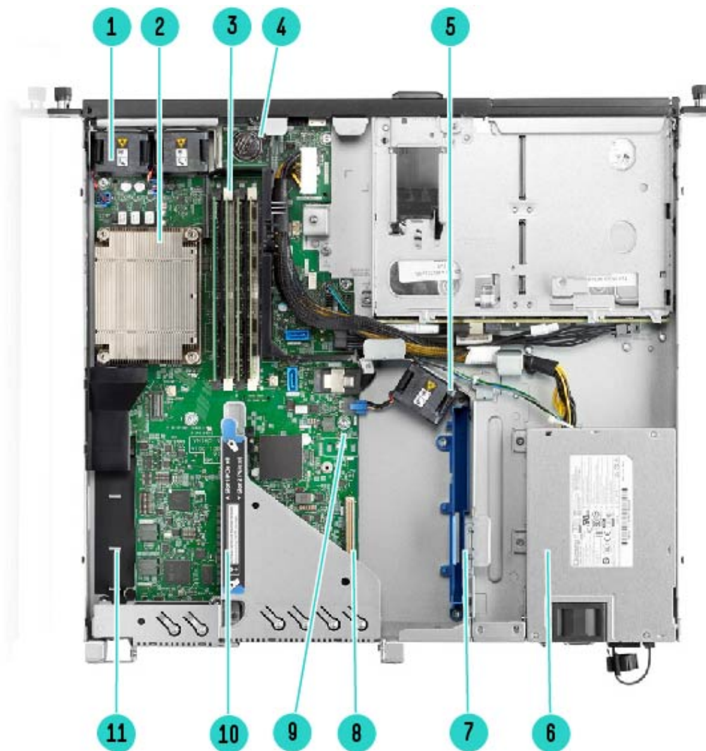
Internal View - Standard for all DL20 Gen10
